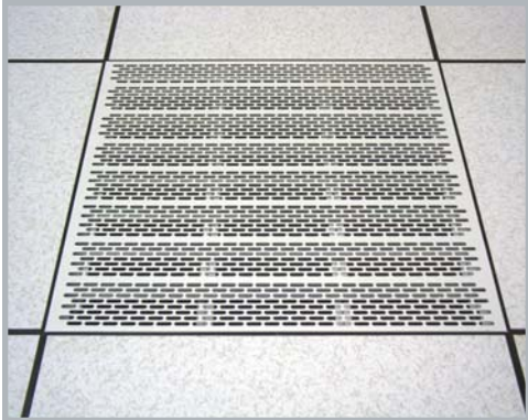
Perf 50 Air Flow Panel
